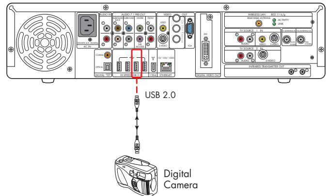
Digital still camera connection (back panel)
